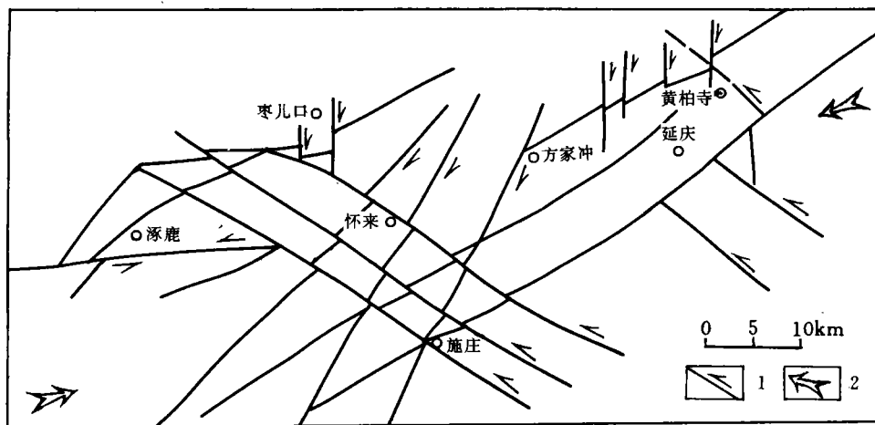
图 10 延-涿地堑盆地上新世—第四纪断裂组合及主压应力方向 Fig. 10 The fault complex and principal compressive stress trend from Pliocene to Quaternary in Yan-zhou graben basin
