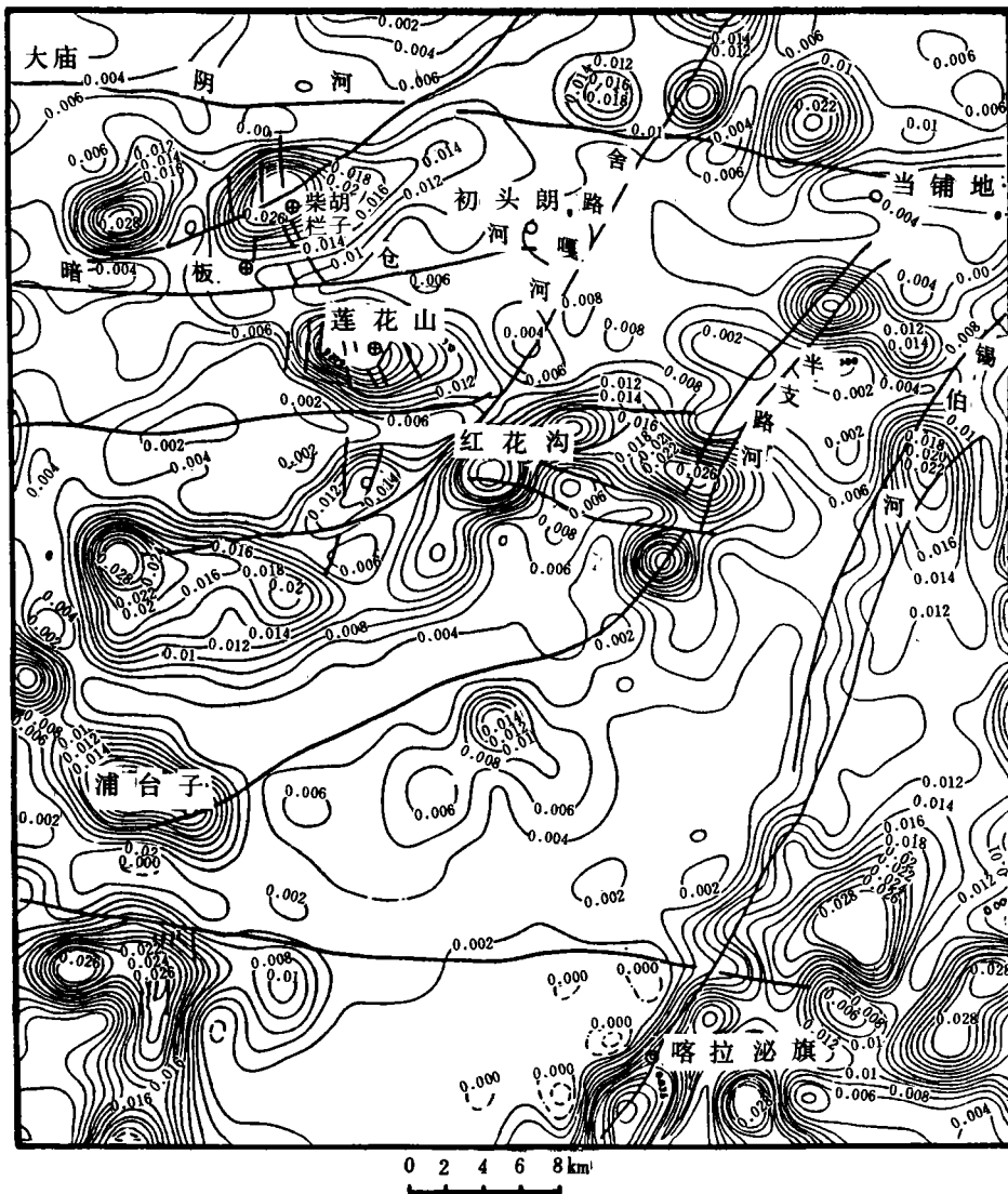
图3 区域激光全息光弹模拟应变能量分级图 Fig. 3 Strain-energy gradational map obtained by the regional photoelastic modelling
