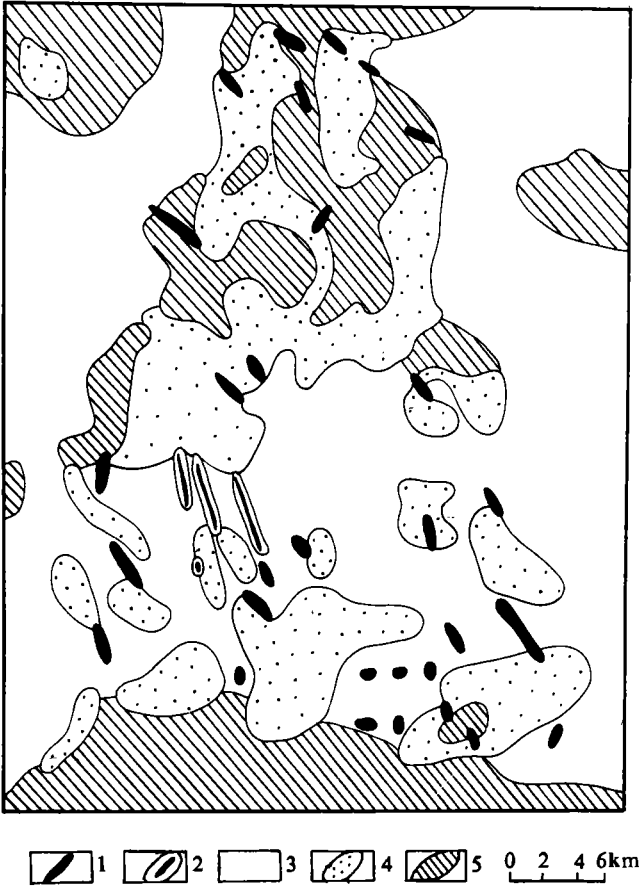
图1 莲花山金矿区同成矿应力场图(平均主应力) Fig. 1 Syn-metallogenic stress field (the mean principal stress) in Lianhuashan gold-ore field 1. 一级区; 2. 二级区; 3. 三级区; 4. 四级区; 5. 五级区
