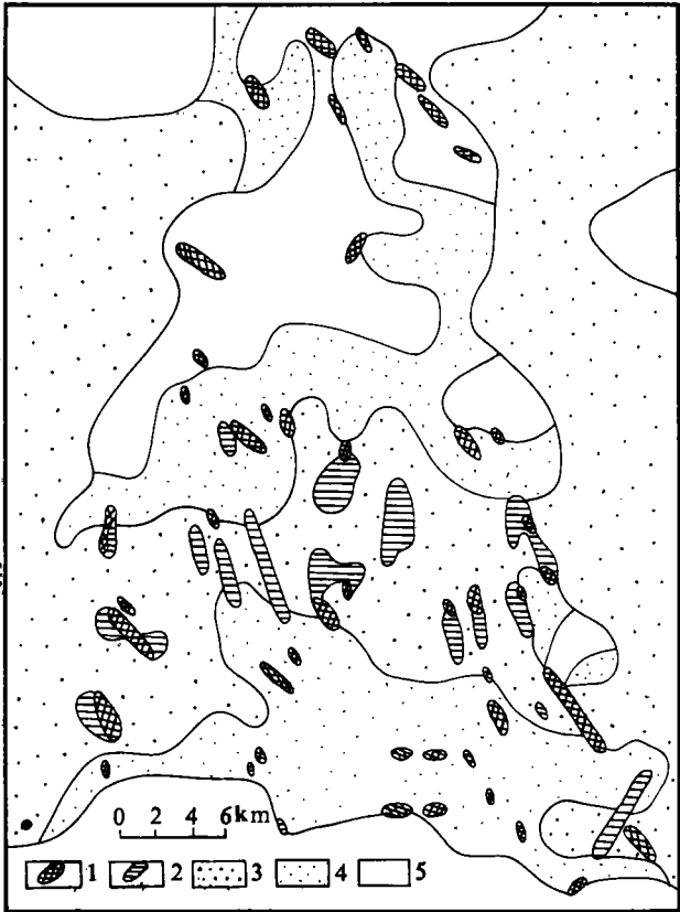
图 2 莲花山金矿区应力降异常图(平均主应力) Fig. 2 Anomaly map of the stress drops (the mean principal stress) in Lianhuashan gold-ore field 1. 一级区;2. 二级区;3. 三级区;4. 四级区;5. 五级区
