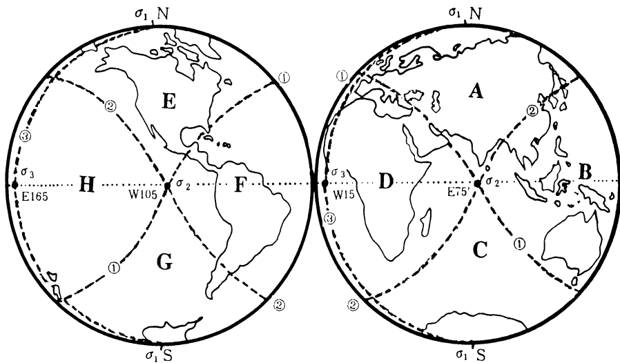
图 4 地球应变椭球体三轴定位及其共轭剪切大圆网络 Fig. 4 Triaxial setting of strain ellipsoid of the Earth and its conjugate shear net of great circle partition
