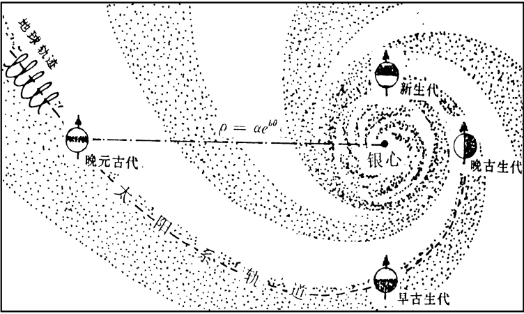
图 6 地球在银河系内的运行状态及其离心力对海陆的控制 Fig. 6 The revolving state of Earth in the galactic system and the ocean-continent distribution by the revolutionary centrifugal force 地球尺度夸大, 球内黑色为大陆, 白色为海洋, 箭头指正北
