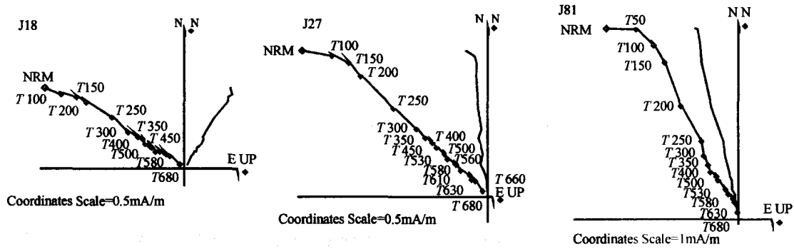
图 4 较场剖面典型样品退磁曲线的特征 Fig.4 Orthogonal projections of progressive thermal demagnetization data of typical samples from the Jiaochang section
