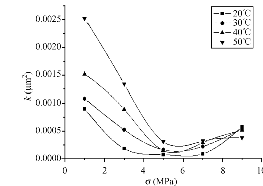
图 6 不同温度下五龙煤样渗透率随有效应力变化曲线 Fig 6 Changing curve of permeability for Wulong coal at different temperatures
