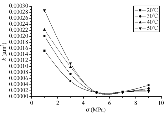
图 3 不同温度下华兴煤样渗透率随有效应力变化曲线 Fig 3 Changing curve of permeability for Huaxing coal at different temperatures
