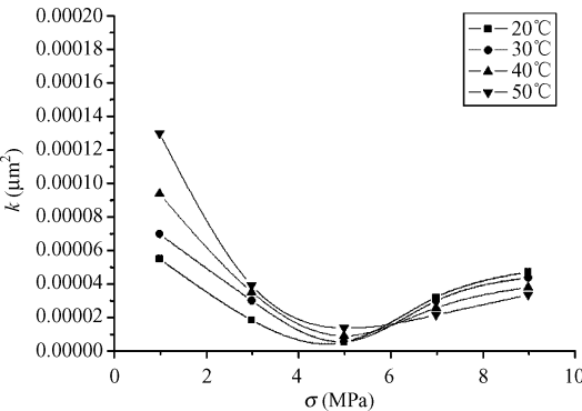
图 5 不同温度下海州煤样渗透率随有效应力变化曲线 Fig 5 Changing curve of permeability for Haizhou coal at different temperatures
