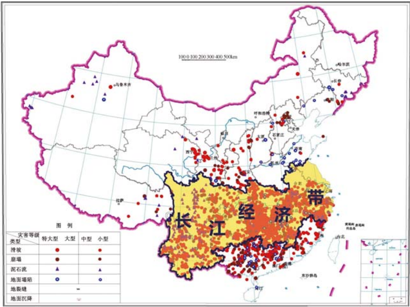
图 1 2015 年度长江经济带地质灾害分布图 (据文献 [4] 修编) Fig. 1 Distribution of geological disasters in the Yangtze River Economic Zone in 2015
