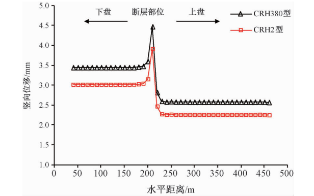
图 9 不同车重下表层土体竖向位移分布曲线 Fig. 9 Distribution curves of vertical displacements of surface soil mass under different train type
