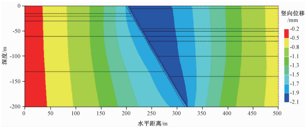
图 10 断层滑动所致竖向位移分布图 Fig. 10 The vertical displacements distribution under the slip of the fault
