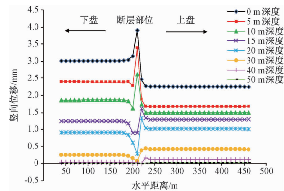
图 7 沿高铁线路方向不同深度土体竖向位移分布情况 Fig. 7 Distribution of vertical displacement of soil mass with different depths under the train load
