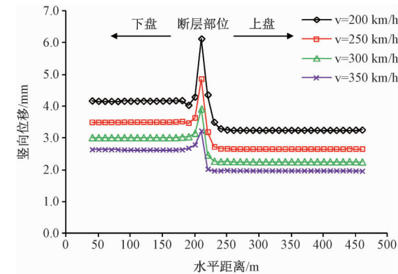
图 8 不同车速下表层土体竖向位移分布曲线 Fig. 8 Distribution curves of vertical displacements of surface soil mass with different train speed
