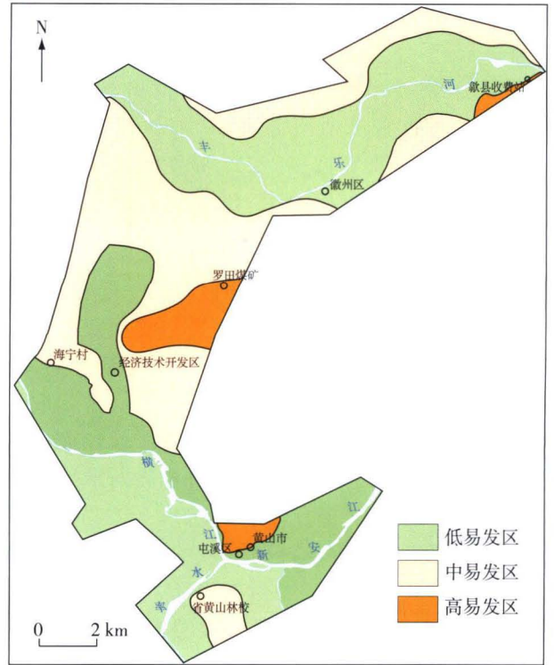
图 6 地质灾害易发分区图 Fig. 6 Map showing division of geological disaster-prone regions
