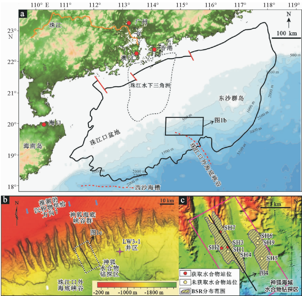
图 1 南海北部陆坡神狐海域区域位置图(a)、海底地貌特征图(b)及 GMGS01 区块内的钻井分布(c) [28] Fig. 1 (a) Location map of the Shenhu Area on the northern continental slope of the South China Sea; (from Ding et al., 2013 [28] ) (b) Bathymetric map of the study area (Shenhu Area) showing nearly seventeen slope-confined submarine canyons; (c) Locations of hydrate drilling sites of GMGS01 in the Shenhu Area
