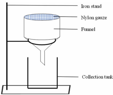
图 1 土壤保水率和流失率测试装置图 Fig. 1 Test equipment for soil water retention and loss rate
