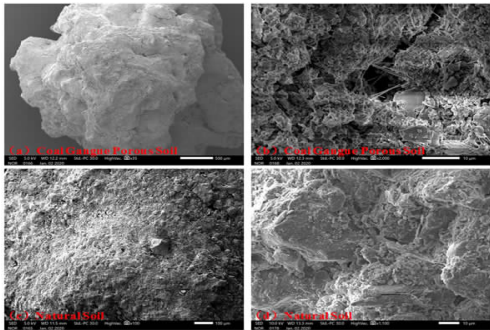
图4 煤矸石多孔土壤与天然土壤 SEM 图 Fig. 4 SEM images of porous soil and natural soil
