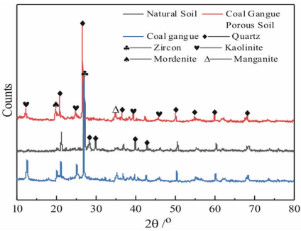
图 3 天然土壤、煤矸石多孔土壤和煤矸石 XRD 对比 Fig. 3 Comparison of XRD of natural soil, coal gangue porous soil and coal gangue
