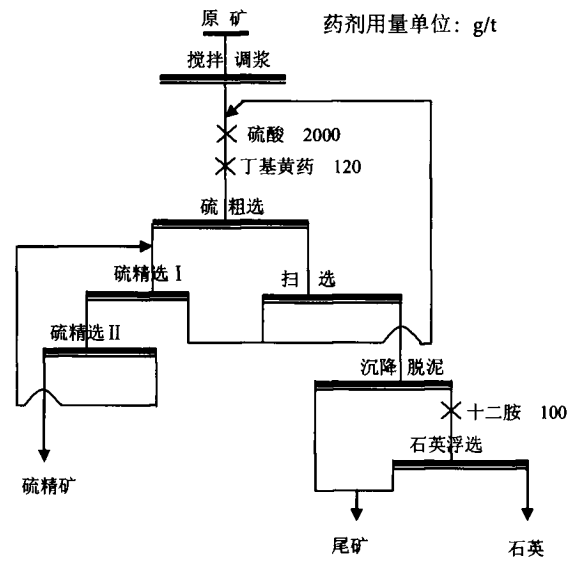
图 6 全流程实验工艺流程及条件 Fig. 6 Technical process and condition of full process test
