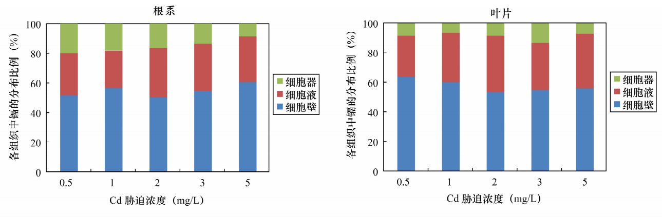
图 1 胁迫浓度对细胞不同组织中镉分布的影响 Fig. 1 Effect of exposure concentration on cadmium distribution in different tissues of cells
