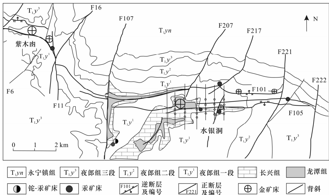
图1 灰家堡背斜金矿田地质图 [4] Fig.1 Geological map of the Huijiabao gold field [4]
