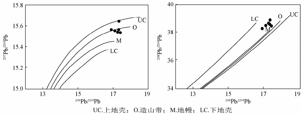
图 2 铅构造模式 Fig.2 Discrimination diagram of Pb isotope composition for tectonic settings
